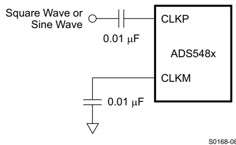
Figure 68. Single-Ended Clock
