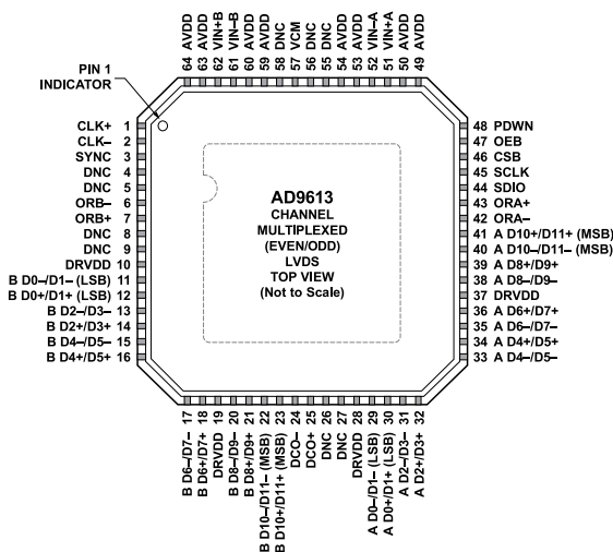
Figure 5. Pin Configuration (Top View) for the LFCSP Channel Multiplexed (Even/Odd) LVDS Mode
