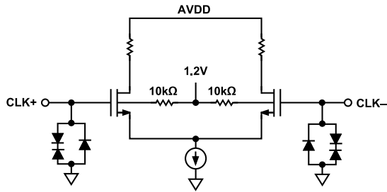
Figure 9. Equivalent Clock Input Circuit
