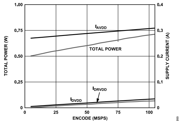
Figure 65. AD9600-105 Power and Current vs. Sample Rate
