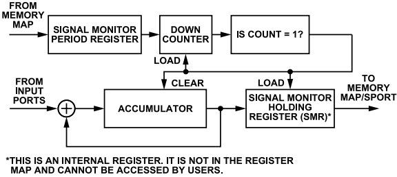
Figure 68. ADC Input RMS Magnitude Monitoring Block Diagram
