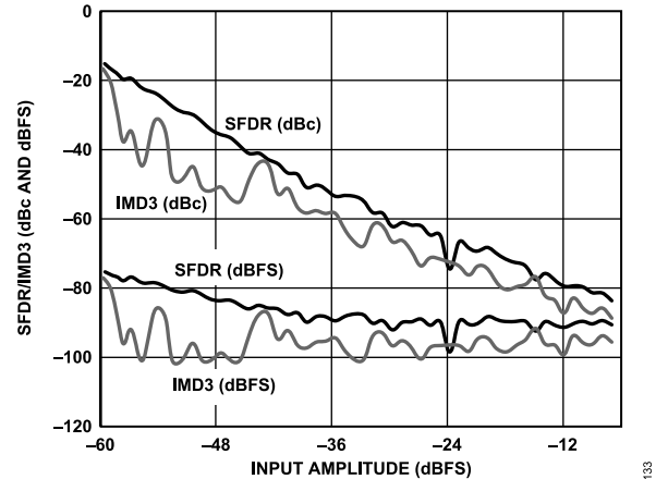
Figure 33. AD9600-150 Two-Tone SFDR/IMD3 vs. Input Amplitude ( A_{IN} ) with f_{IN1} = 29.1 MHz, f_{IN2} = 32.1 MHz, f_S = 150 MSPS
