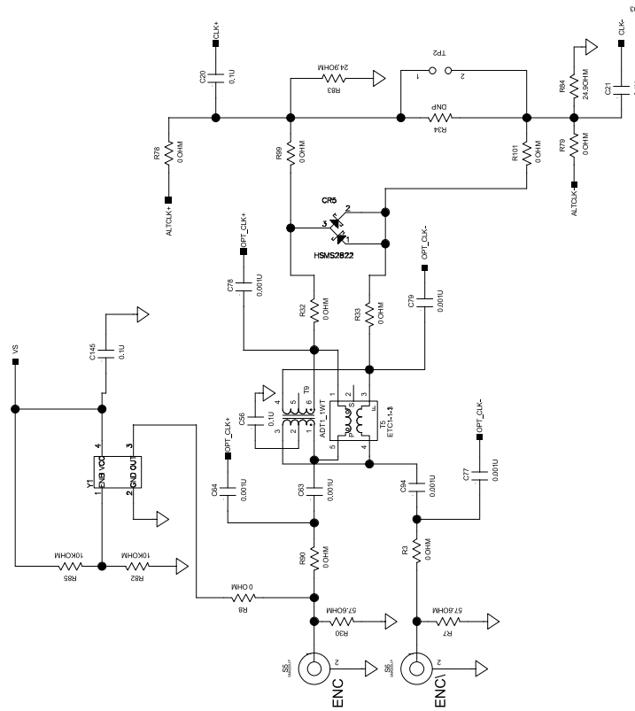
Figure 76. Evaluation Board Schematic, DUT Clock Input
