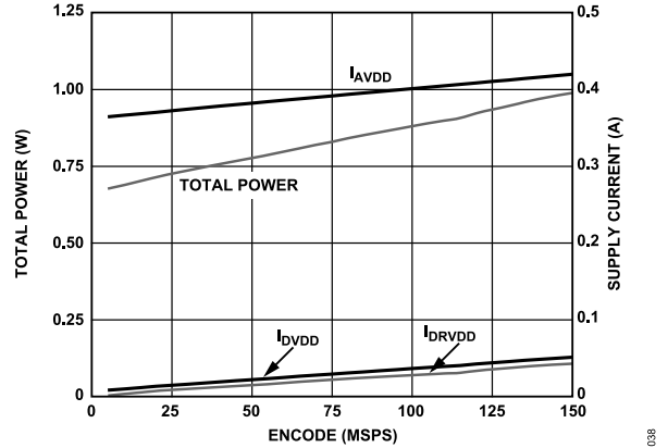
Figure 63. AD9600-150 Power and Current vs. Sample Rate
