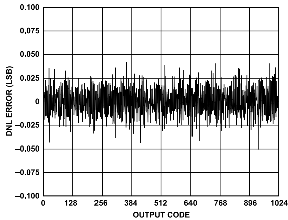
Figure 42. AD9600 DNL with f_{IN1} = 10.3 MHz
