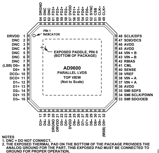
Figure 7. Interleaved Parallel LVDS Mode Pin Configuration (Top View)
