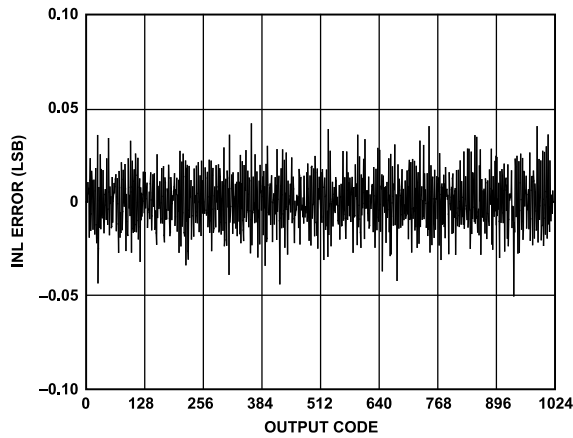
Figure 41. AD9600 INL with f_{IN1} = 10.3 MHz
