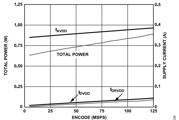
Figure 64. AD9600-125 Power and Current vs. Sample Rate
