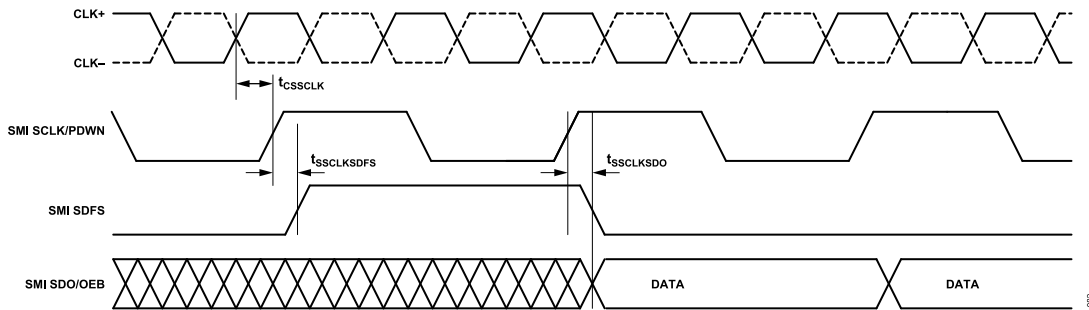
Figure 5. Signal Monitor SPORT Output Timing (Divide-by-2 Mode)
