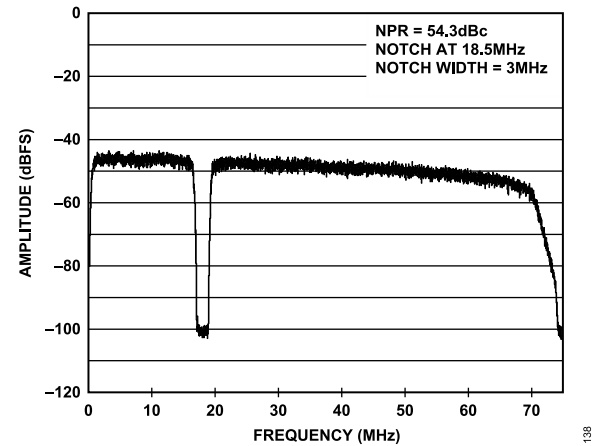
Figure 38. AD9600-150 Noise Power Ratio (NPR)
