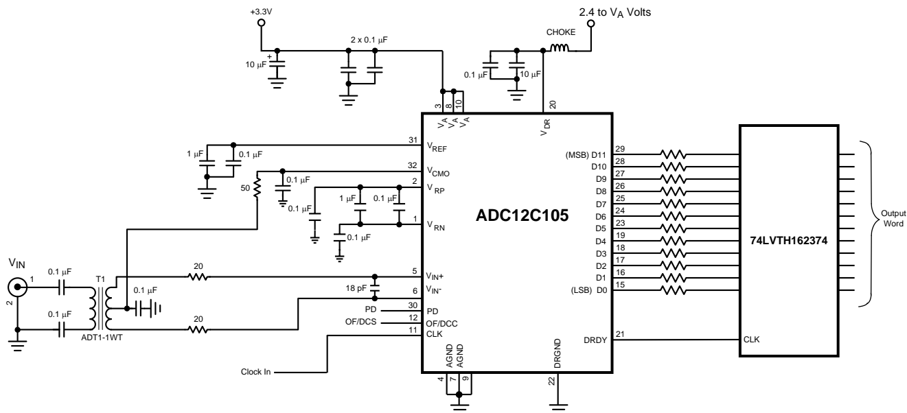
Figure 34. Application Circuit
