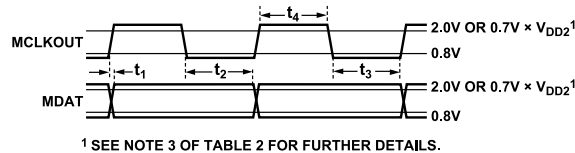
Figure 2. Data Timing
