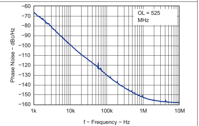
Figure 70. Open Loop VCO Phase Noise
