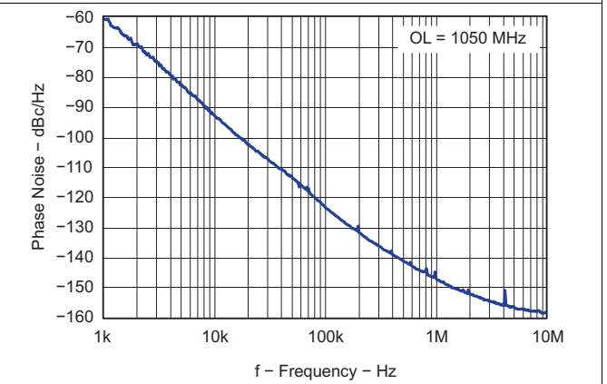
Figure 68. Open Loop VCO Phase Noise
