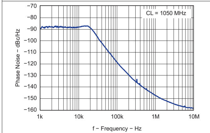
Figure 67. Closed Loop VCO Phase Noise
