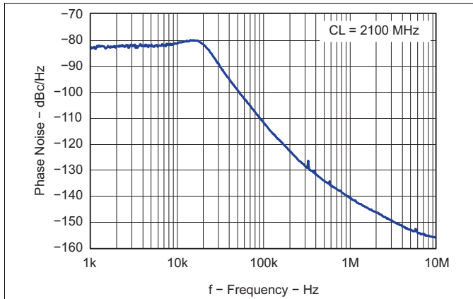
Figure 65. Closed Loop VCO Phase Noise
