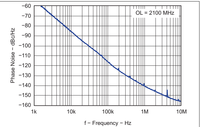
Figure 66. Open Loop VCO Phase Noise
