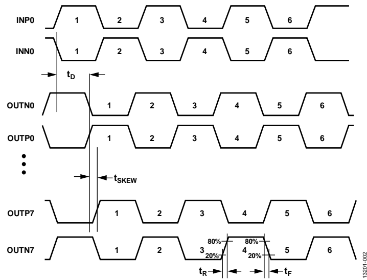
Figure 2. Timing Diagram
