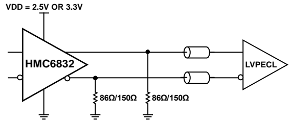
Figure 51. LVPECL Output DC Termination Interface (86 Ohm Termination Can Be Used at 2.5 V Only)
