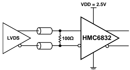
Figure 49. LVDS DC-Coupled Input Interface
