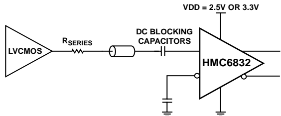
Figure 48. LVCMOS AC-Coupled Input Interface
