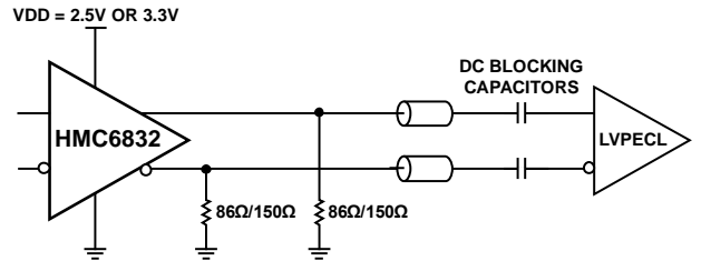
Figure 52. LVPECL Output AC Termination Interface (86 Ohm Termination Can Be Used at 2.5 V Only)
