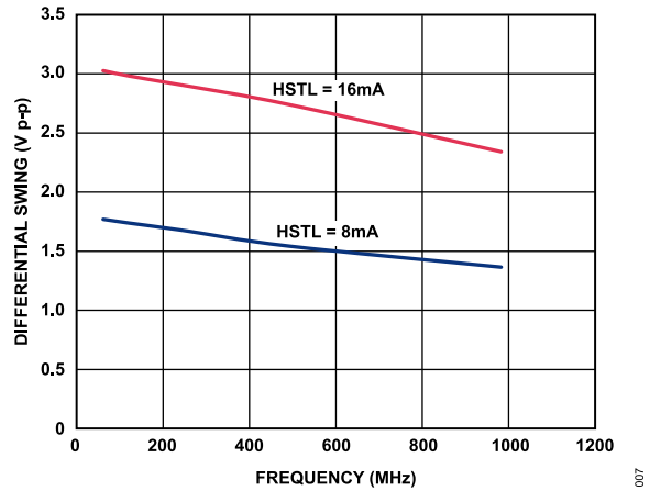
Figure 7. Differential Voltage Swing vs. Frequency; HSTL Mode, 16 mA and 8 mA
