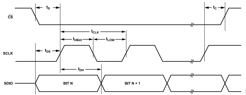
Figure 43. Serial Control Port Timing—Write
