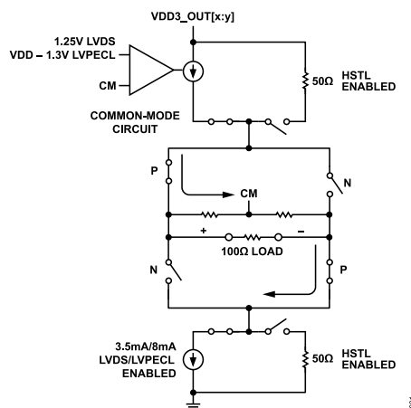
Figure 26. Multimode Driver
