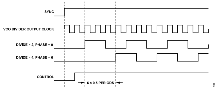
Figure 28. Clock Output Synchronization Timing Diagram
