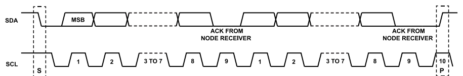
Figure 32. Data Transfer Process (Main Write Mode, 2-Byte Transfer)
