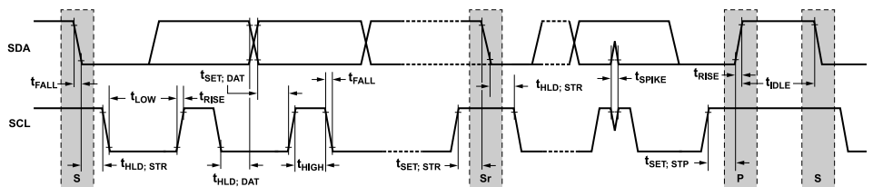
Figure 34. I 2 C Serial Port Timing
