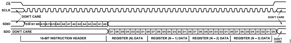
Figure 39. Serial Control Port Read—MSB First, 16-Bit Instruction, Four Bytes of Data
