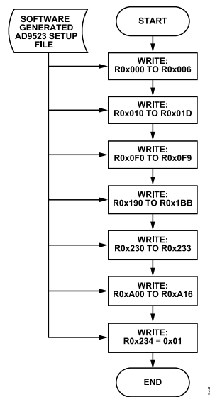
Figure 45. Subprocess: Write Registers from Setup File
