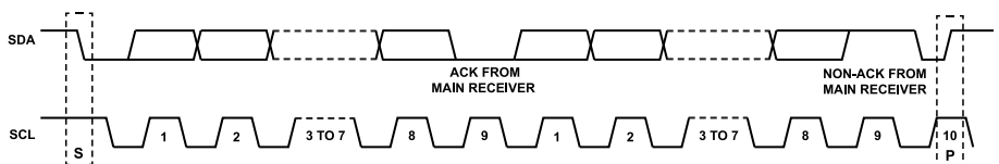
Figure 33. Data Transfer Process (Main Read Mode, 2-Byte Transfer)
