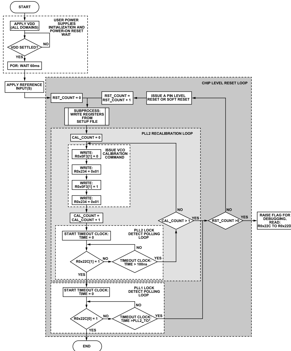
Figure 44. AD9523 Device Initialization
