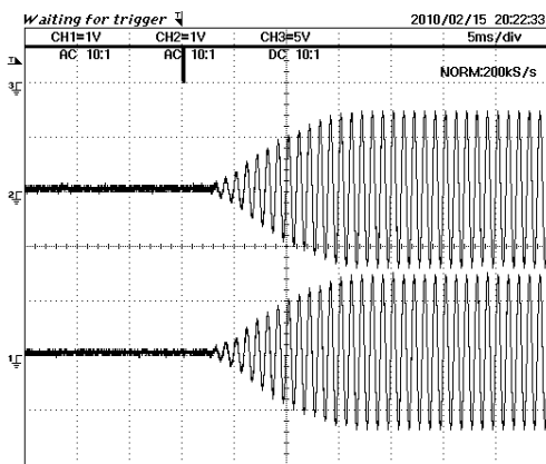
Figure 19. Advanced Switch 1
