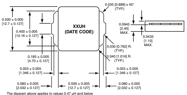
The diagram above applies to values 0.47 μH and below
