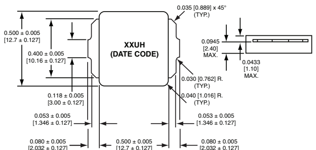
The diagram above applies to values 0.68 μH and above
