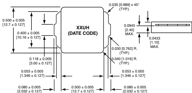
The diagram above applies to values 0.68 µH and above
