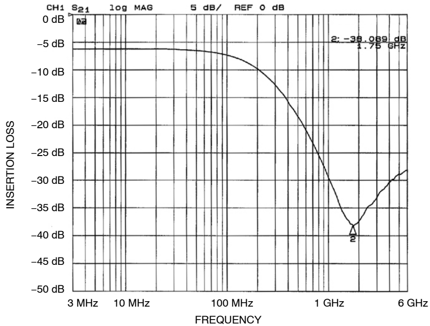
Figure 5. Insertion Loss vs. Frequency (FILTER1 Input to GND, CM1630-06DE)
