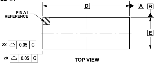
WLCSP20, 4.00x1.46 CASE 567BZ ISSUE O
