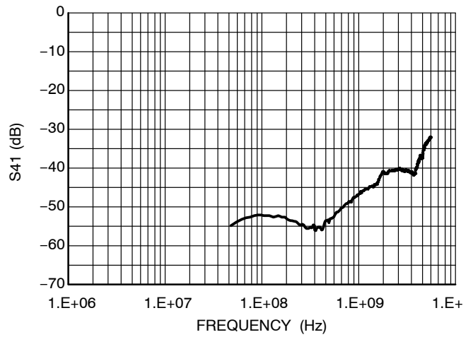
Figure 4. Typical Analog Crosstalk
