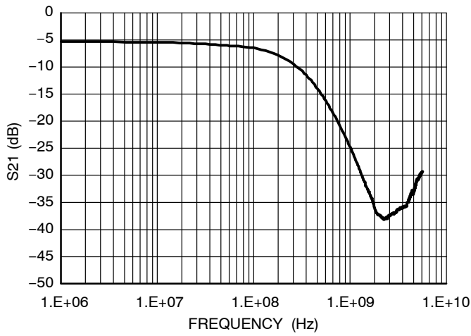
Figure 3. Typical Insertion Loss Characteristic
