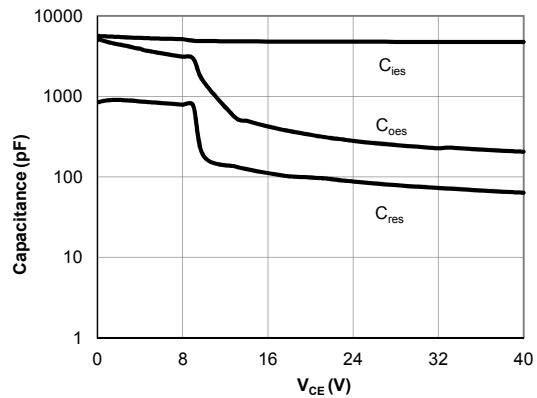
Figure 8: Capacitance Characteristic
