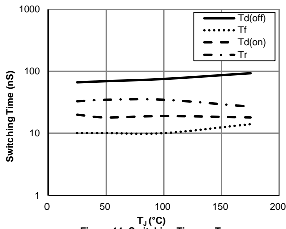
Figure 14: Switching Time vs. T_J ( V_{GE}=15\text{V}, V_{CE}=400\text{V}, I_C=20\text{A}, R_g=15\Omega )
