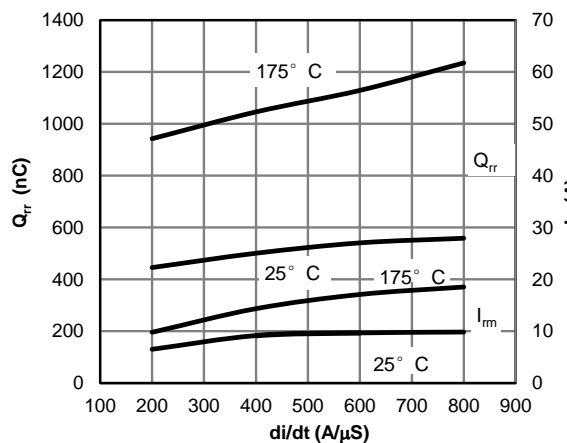
Fig 23: Diode Reverse Recovery Charge and Peak Current vs. di/dt ( V_{GE}=15V, V_{CE}=400V, I_F=10A )
