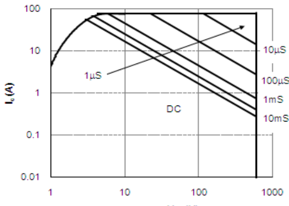
Fig 9: Forward Bias Safe Operating Area ( T_C=25C, V_{GE}=15V )
