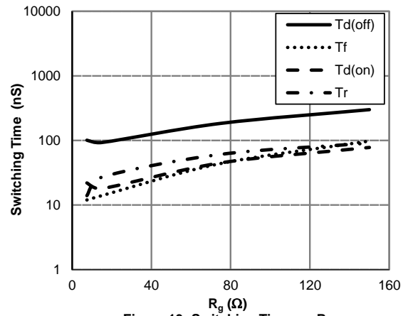
Figure 13: Switching Time vs. R_g ( T_J=175^\circ\text{C}, V_{GE}=15\text{V}, V_{CE}=400\text{V}, I_C=20\text{A} )
