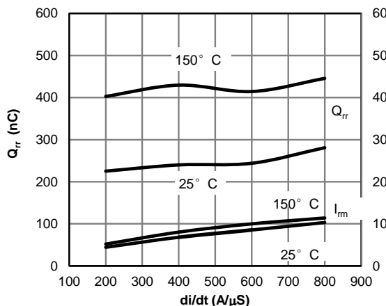
Figure 25: Diode Reverse Recovery Charge and Peak Current vs. di/dt ( V_{GE}=15V, V_{CE}=400V, I_F=5A )
