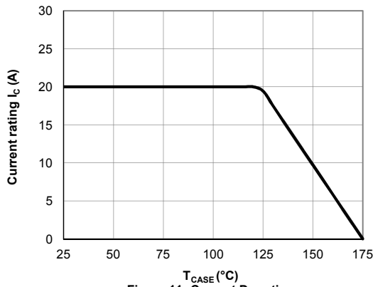
Figure 11: Current De-rating
