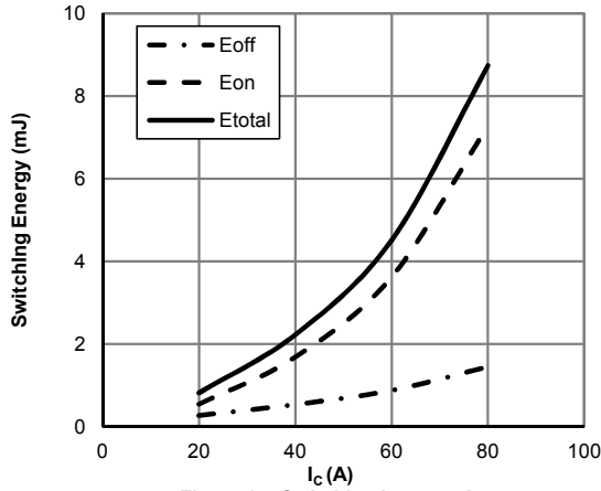
Figure 14: Switching Loss vs. I_C ( T_J=150^\circ\text{C} , V_{GE}=15\text{V} , V_{CE}=400\text{V} , R_\theta=7.5\Omega )
