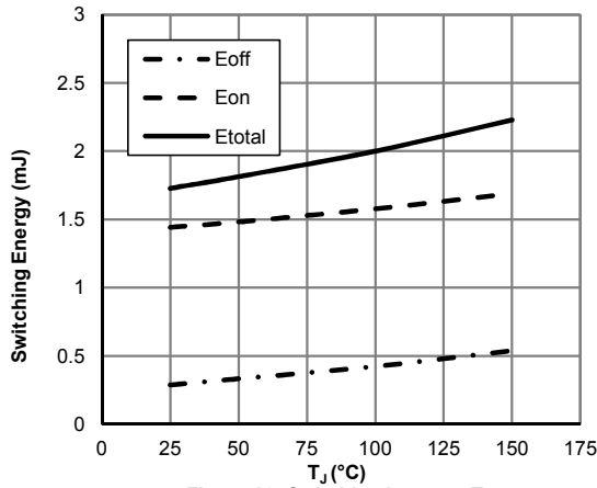
Figure 16: Switching Loss vs. T_J ( V_{GE}=15\text{V} , V_{CE}=400\text{V} , I_C=40\text{A} , R_\theta=7.5\Omega )
