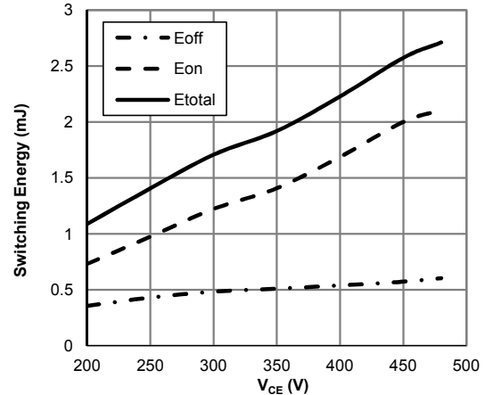
Figure 17: Switching Loss vs. V_{CE} ( T_J=150^\circ\text{C} , V_{GE}=15\text{V} , I_C=40\text{A} , R_\theta=7.5\Omega )
