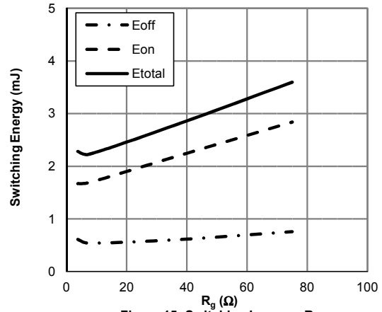
Figure 15: Switching Loss vs. R_\theta ( T_J=150^\circ\text{C} , V_{GE}=15\text{V} , V_{CE}=400\text{V} , I_C=40\text{A} )
