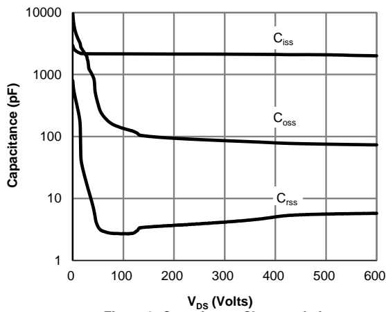
Figure 9: Capacitance Characteristics
