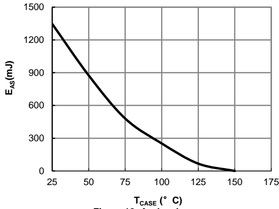
Figure 12: Avalanche energy
