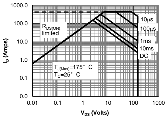
Figure 9: Maximum Forward Biased V_{GS} > \text{or equal to } 6V
