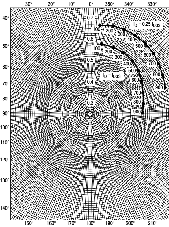
Figure 13. S_{11g}
