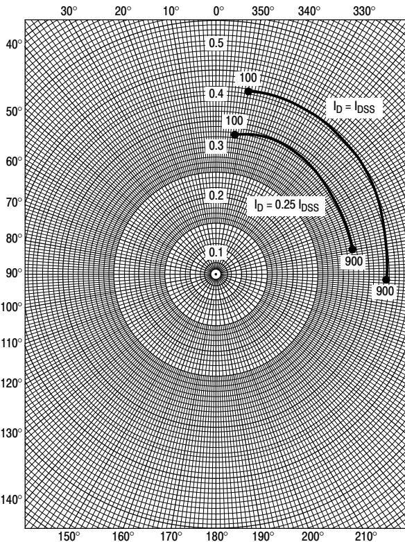
Figure 15. S_{21g}
