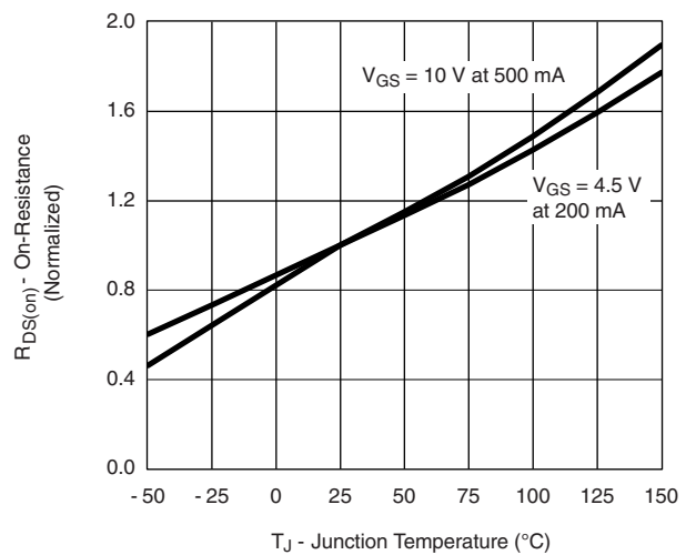
V_{GS} = 10 V at 500 mA 4.5 V at 200 mA On-Resistance vs. Junction Temperature
