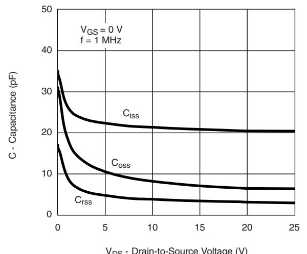
V_{GS} = 0 V f = 1 MHz Capacitance
