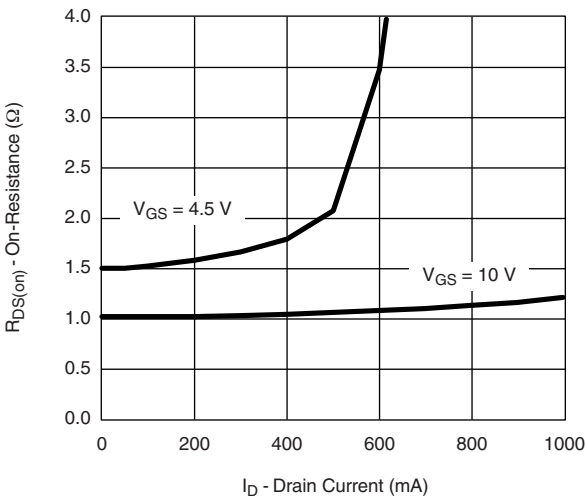
V_{GS} = 4.5 V 10 V On-Resistance vs. Drain Current
