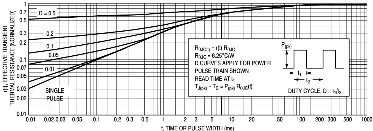
Figure 3. Thermal Response
