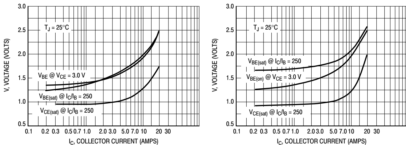
Figure 9. "On" Voltages
