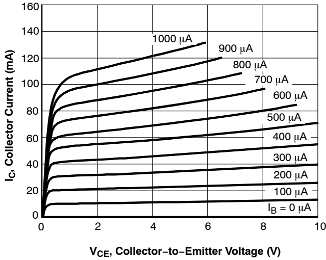
Figure 1. I_C - V_{CE}
