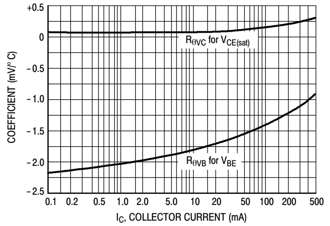
Figure 6. Temperature Coefficients
