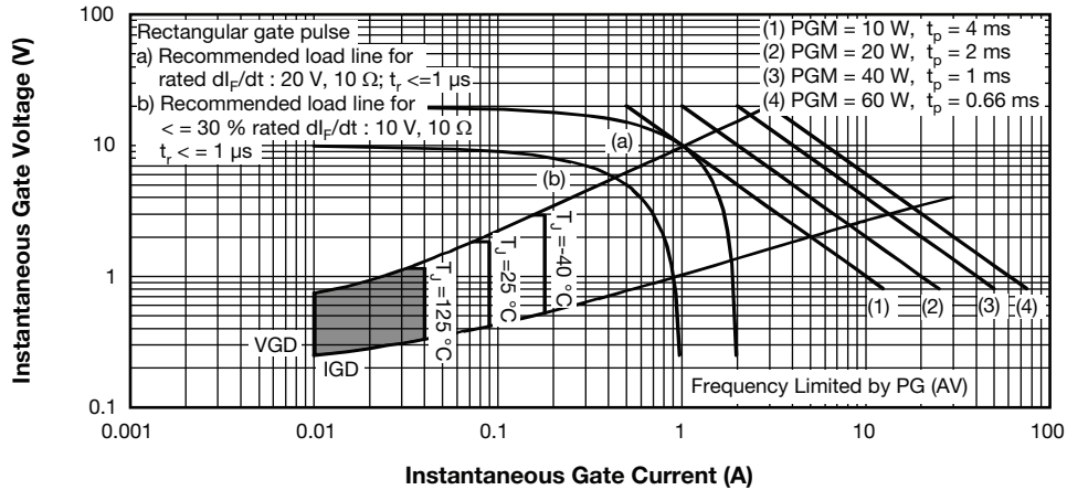
Fig. 9 - Gate Characteristics
