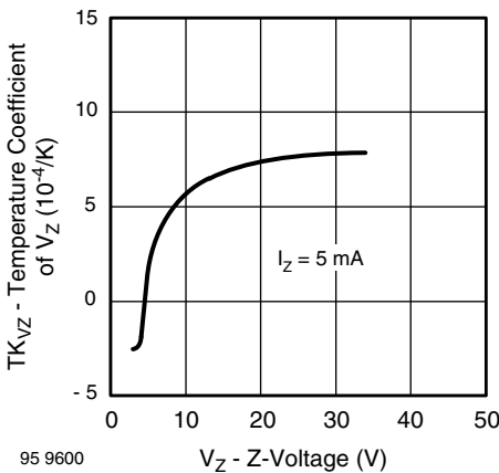
Fig. 3 - Typical Temperature Coefficient of V Z vs. Z-Voltage
