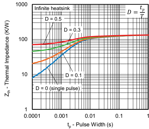
Fig. 7 - Typical Thermal Response
