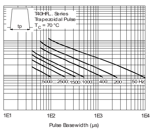
Fig. 37 - Frequency Characteristics
