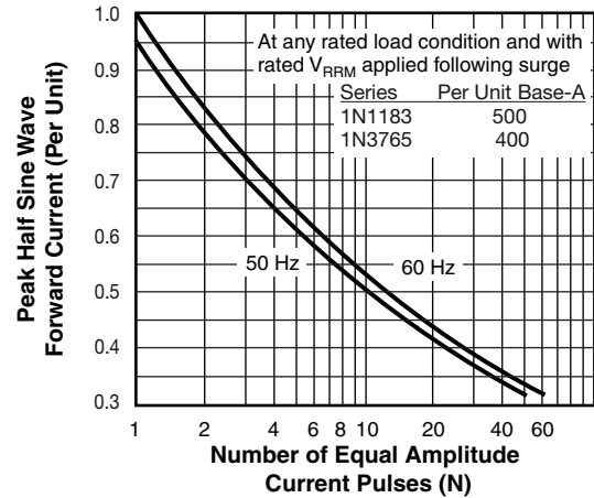
Fig. 5 - Maximum Non-Repetitive Surge Current vs. Number of Current Pulses, 1N1183 and 1N3765 Series
