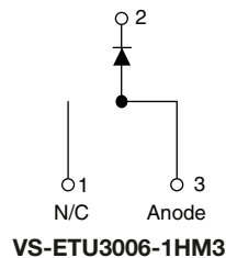
TO-262AA
