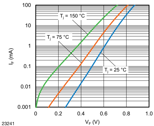
23241 Fig. 2 - Forward Current vs. Forward Voltage
