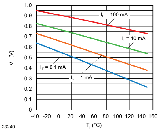
23240 Fig. 1 - Typical Forward Voltage vs. Junction Temperature
