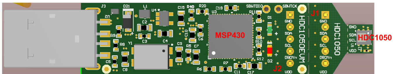
Figure 1. HDC1050EVM
