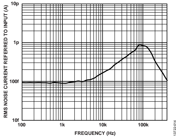
Figure 10. Noise Bandwidth/Peaking
