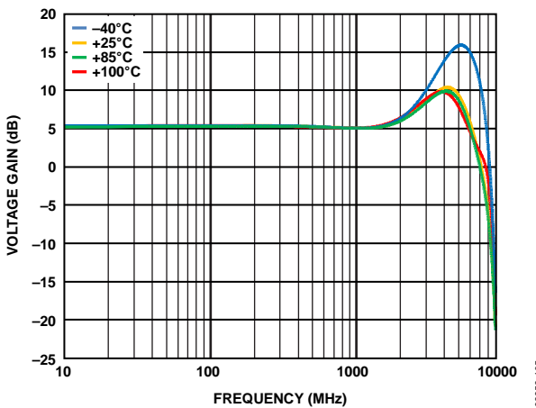
Figure 5. Gain vs. Frequency Response for 200 \Omega Differential Load, A_V = 6\text{ dB} , Four Temperatures, V_{POS} = 5\text{ V} , 25^\circ\text{C}
