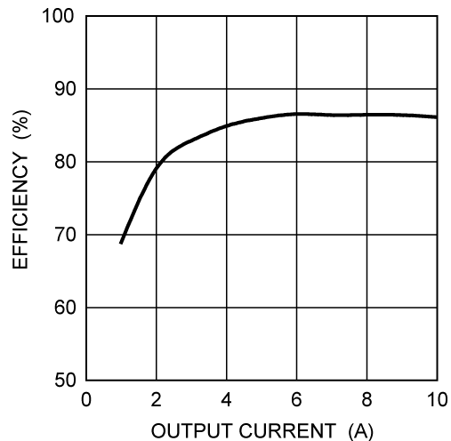
Figure 2-1. Efficiency for V_{IN} = 12\text{ V}
