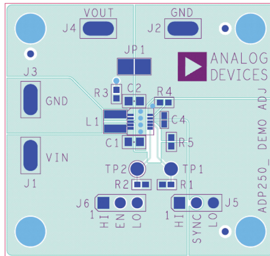
Figure 1. ADP2503/ADP2504 Adjustable Evaluation Board
