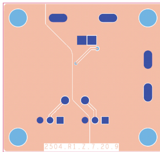
Figure 10. Bottom Layer, Recommended Layout
