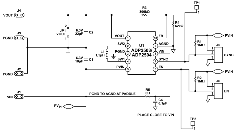
Figure 8. ADP2503/ADP2504 Adjustable Evaluation Board Schematic
