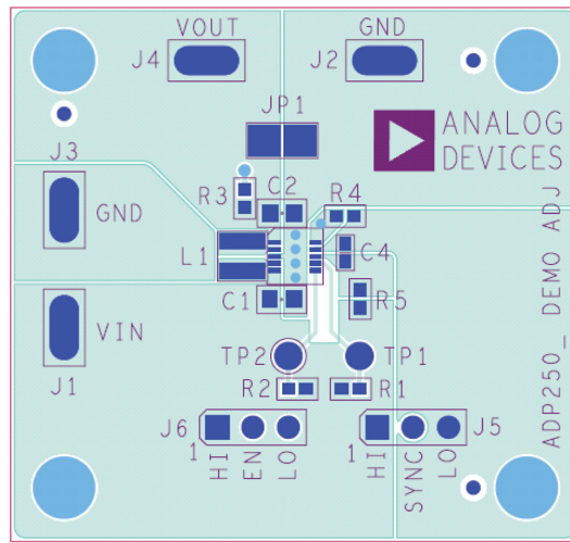
Figure 9. Top Layer, Recommended Layout
