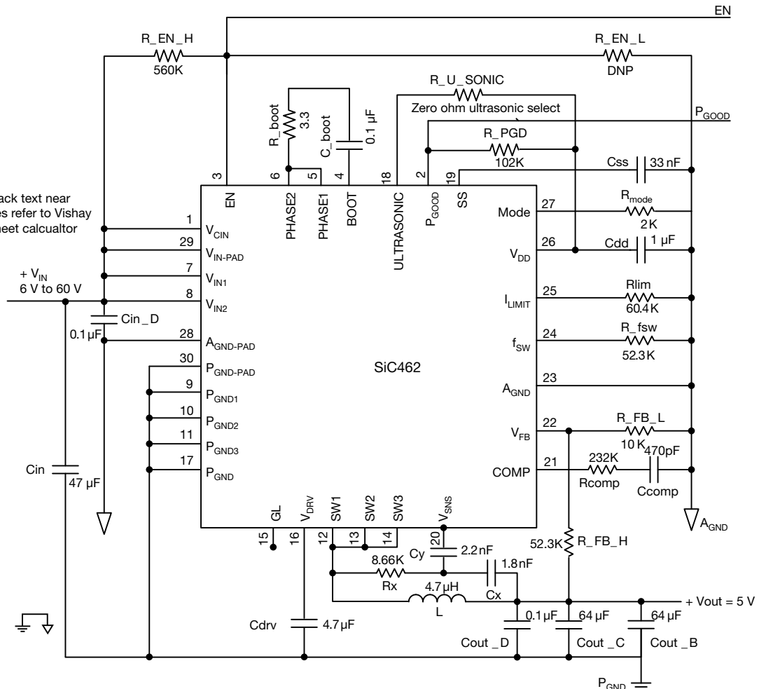
Fig. 10 - SiC462 Configured for 6 V to 60 V Input, 5 V Output at 6 A, 500 kHz Operation with Ultrasonic Power Save Mode Enabled all Ceramic Output Capacitance Design
