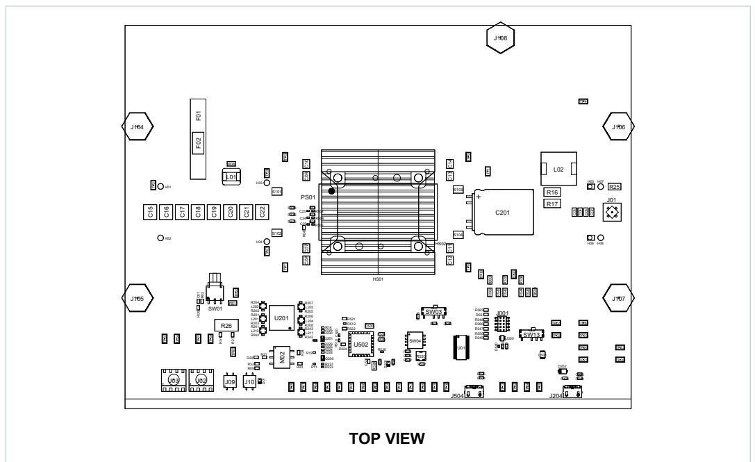
Figure 6 DCM4623 evaluation board assembly drawing, top side
