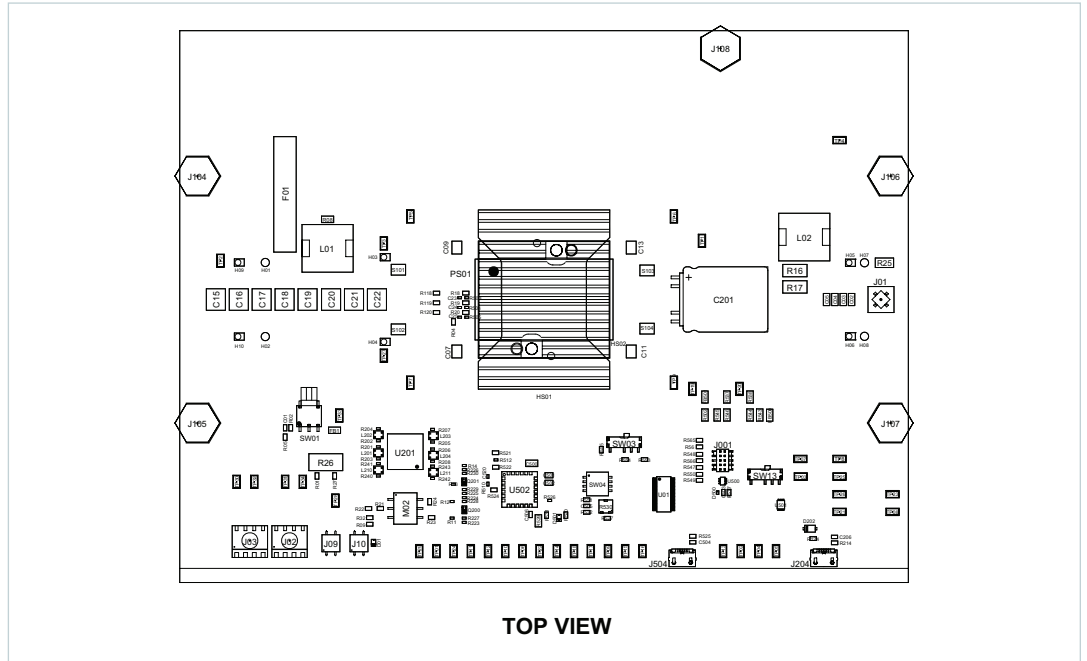
Figure 5 DCM3623 evaluation board, assembly drawing, top side
