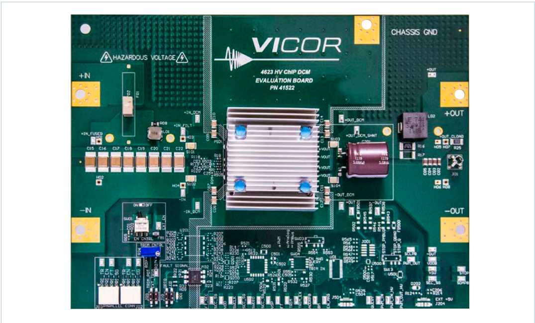
Figure 2 DCM4623 evaluation board photo, top side
