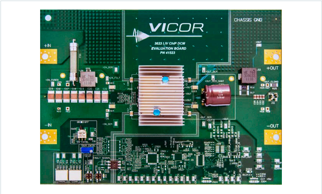
Figure 1 DCM3623 evaluation board photo, top side
