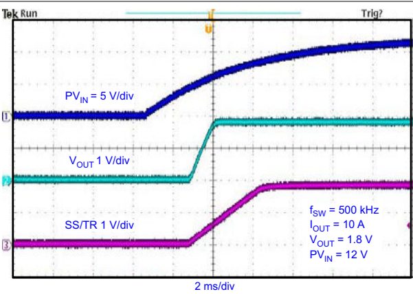
Figure 5-8. LMZ31710EVM Start-Up Waveforms
