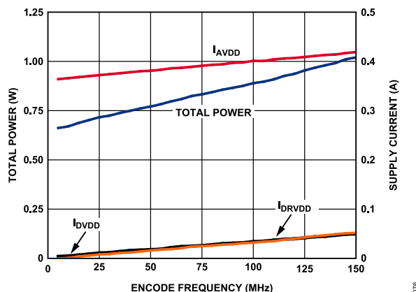
Figure 63. AD9640-150 Power and Current vs. Clock Frequency
