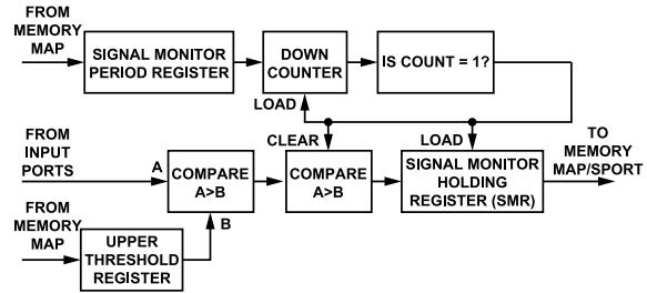
Figure 70. ADC Input Threshold Crossing Block Diagram
