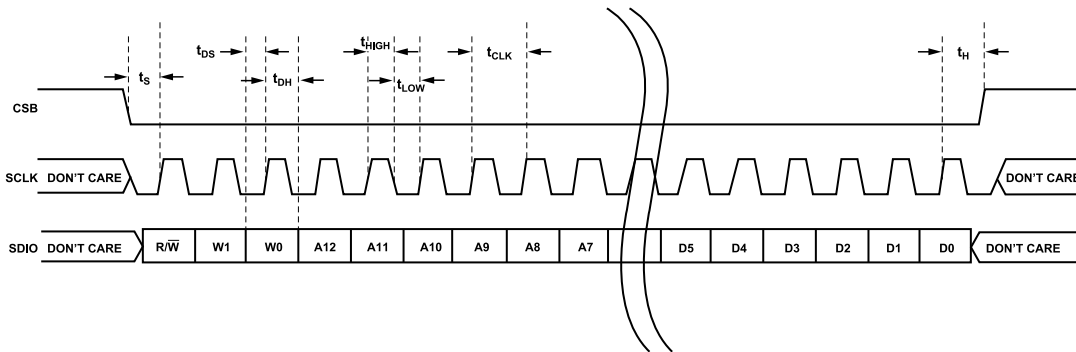
Figure 73. Serial Port Interface Timing Diagram
