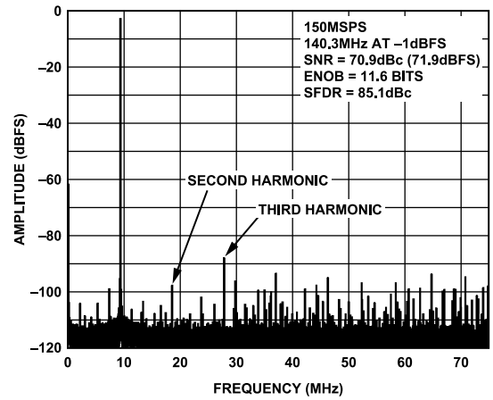
Figure 19. AD9640-150 Single-Tone FFT with f_{IN} = 140.3 MHz
