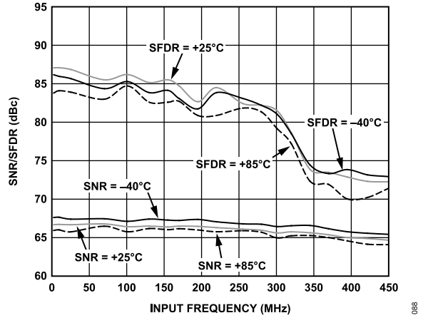
Figure 31. AD9640-150 Single-Tone SNR/SFDR vs. Input Frequency ( f_{IN} ) and Temperature with 1 V p-p Full Scale
