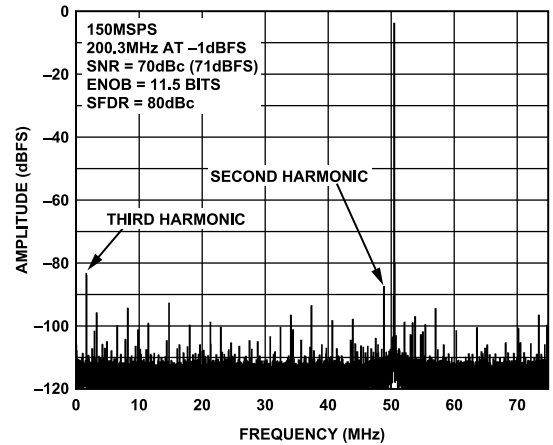
Figure 20. AD9640-150 Single-Tone FFT with f_{IN} = 200.3 MHz
