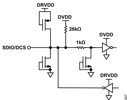
Figure 11. Equivalent SDIO/DCS or SMI SDFS Circuit
