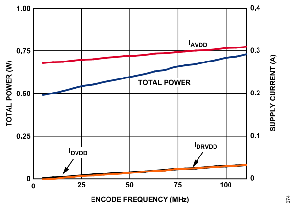
Figure 65. AD9640-105 Power and Current vs. Clock Frequency
