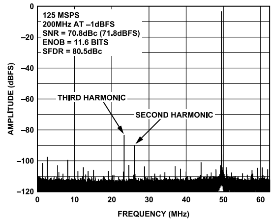
Figure 27. AD9640-125 Single-Tone FFT with f_{IN} = 200 MHz
