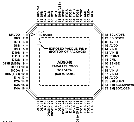
Figure 6. Pin Configuration, LFCSP Parallel CMOS (Top View)
