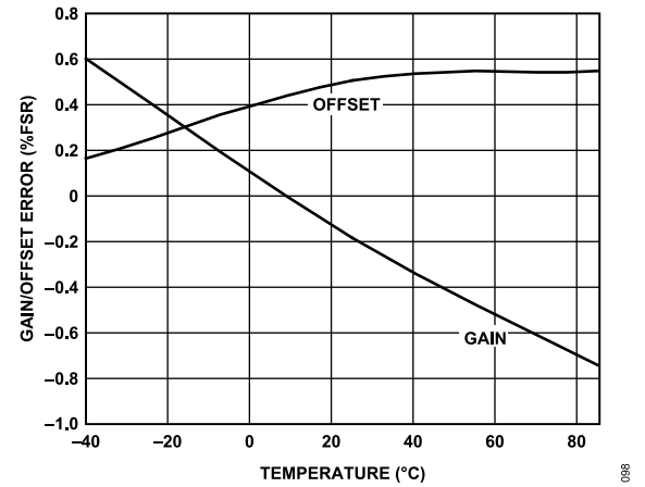
Figure 32. AD9640 Gain and Offset vs. Temperature
