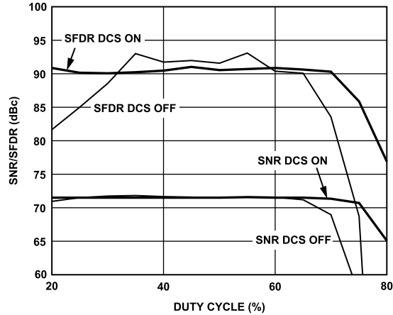
Figure 43. AD9640 SNR/SFDR vs. Duty Cycle with f_{IN} = 10.3 MHz
