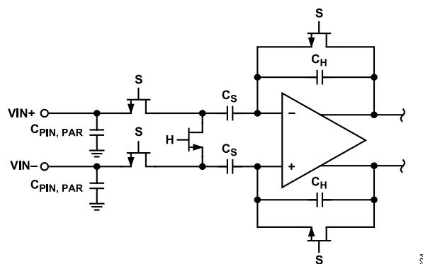
Figure 45. Switched-Capacitor SHA Input
