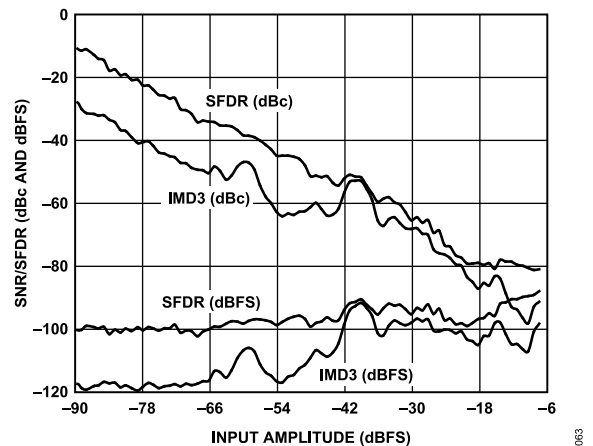
Figure 33. AD9640-150 Two-Tone SFDR/IMD3 vs. Input Amplitude ( A_{IN} ) with f_{IN1} = 29.1 MHz, f_{IN2} = 32.1 MHz, f_S = 150 MSPS
