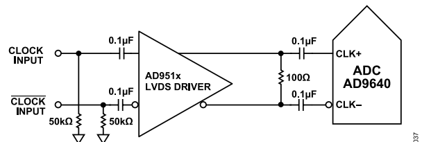
Figure 59. Differential LVDS Sample Clock (Up to 625 MHz)
