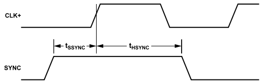
Figure 4. SYNC Input Timing Requirements
