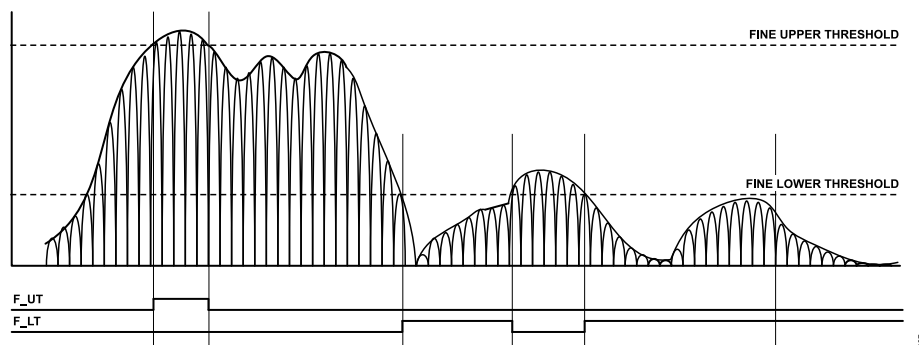
Figure 67. Threshold Settings for F_UT and F_LT
