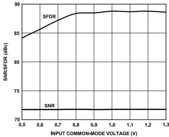
Figure 44. AD9640 SNR/SFDR vs. Input Common Mode Voltage (VCM) with f_{IN} = 30 MHz
