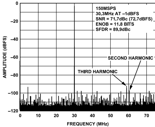
Figure 17. AD9640-150 Single-Tone FFT with f_{IN} = 30.3 MHz
