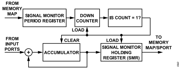
Figure 69. ADC Input RMS Magnitude Monitoring Block Diagram
