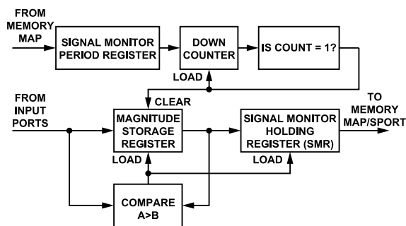
Figure 68. ADC Input Peak Detector Block Diagram.
