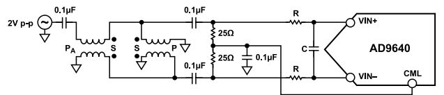
Figure 49. Differential Double Balun Input Configuration
