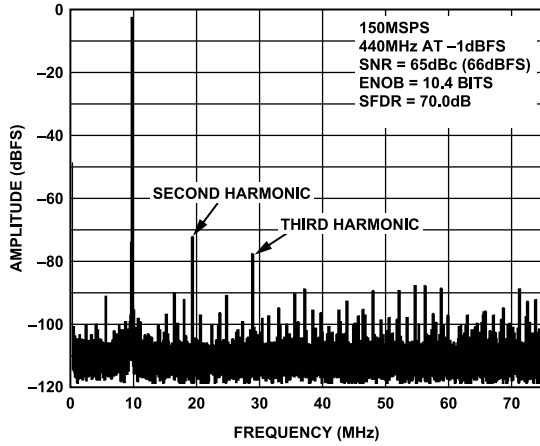
Figure 22. AD9640-150 Single-Tone FFT with f_{IN} = 440 MHz
