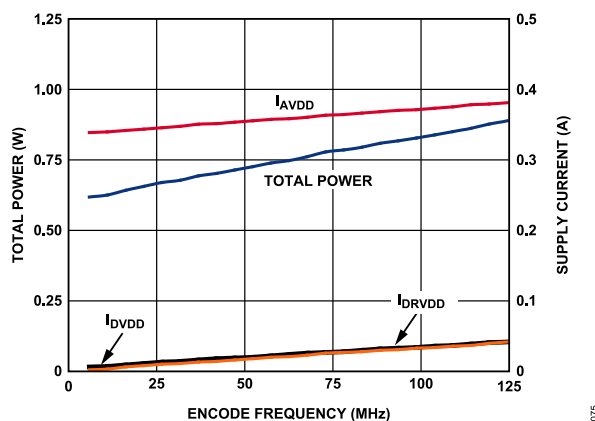
Figure 64. AD9640-125 Power and Current vs. Clock Frequency
