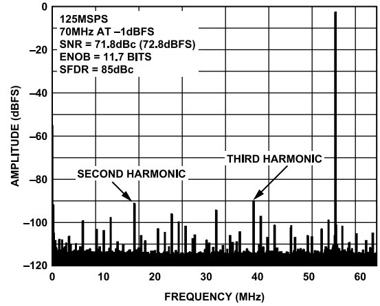
Figure 25. AD9640-125 Single-Tone FFT with f_{IN} = 70 MHz
