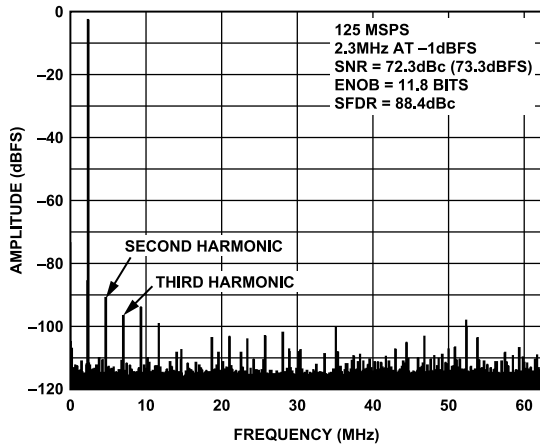
Figure 23. AD9640-125 Single-Tone FFT with f_{IN} = 2.3 MHz
