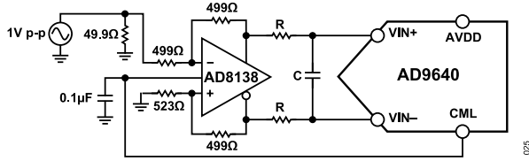
Figure 46. Differential Input Configuration Using the AD8138
