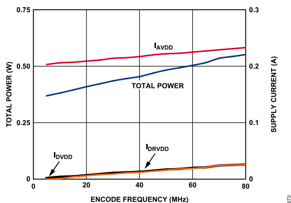
Figure 66. AD9640-80 Power and Current vs. Clock Frequency
