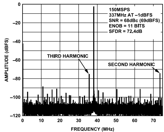
Figure 21. AD9640-150 Single-Tone FFT with f_{IN} = 337 MHz
