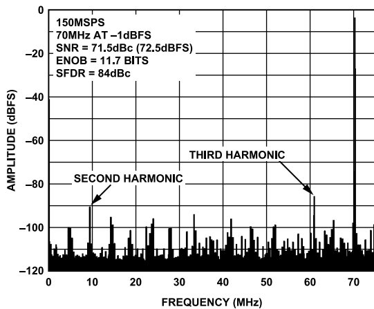
Figure 18. AD9640-150 Single-Tone FFT with f_{IN} = 70 MHz
