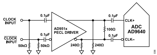
Figure 58. Differential PECL Sample Clock (Up to 625 MHz)
