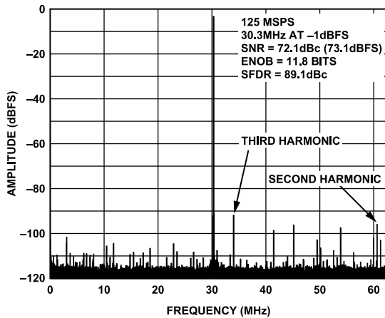
Figure 24. AD9640-125 Single-Tone FFT with f_{IN} = 30.3 MHz
