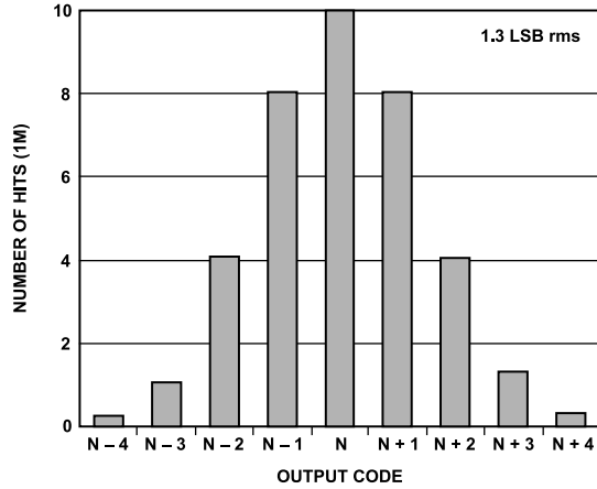
Figure 40. AD9640 Grounded Input Histogram
