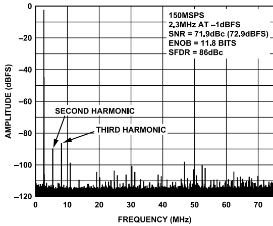
Figure 16. AD9640-150 Single-Tone FFT with f_{IN} = 2.3 MHz
