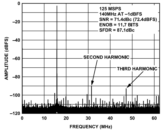
Figure 26. AD9640-125 Single-Tone FFT with f_{IN} = 140 MHz
