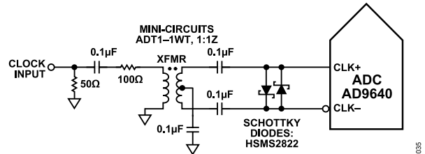
Figure 56. Transformer Coupled Differential Clock (Up to 200 MHz)
