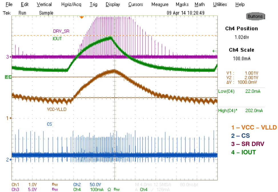
Figure 20. V_{IN} = 230 \text{ V}_{AC} , I_{OUT} = 22\text{--}202 \text{ mA} , SR Controller Driver Output Voltage is Modulated Accordingly to Load Current through LLD Pin. Regulation Range is 1 to 2 V. NCP4305 Enters Disable Mode where its Consumption Significantly Decreases when V_{CC} - V_{LLD} is below 1 V
