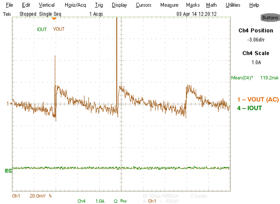
Figure 9. V_{IN} = 230 V_{AC} , I_{OUT} = 100 \text{ mA} , Primary Controller is in Skip Mode, \Delta V_{OUTPK-PK} = 30 \text{ mV}
