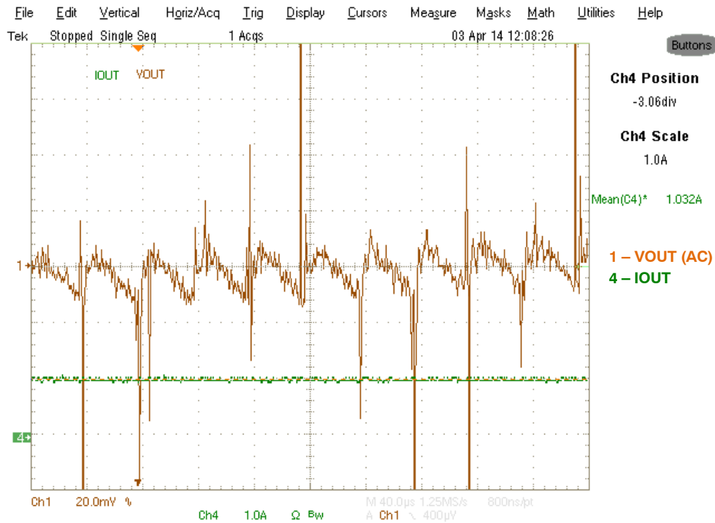
Figure 10. V_{IN} = 230 V_{AC} , I_{OUT} = 1 \text{ A} , \Delta V_{OUTPK-PK} = 20 \text{ mV}
