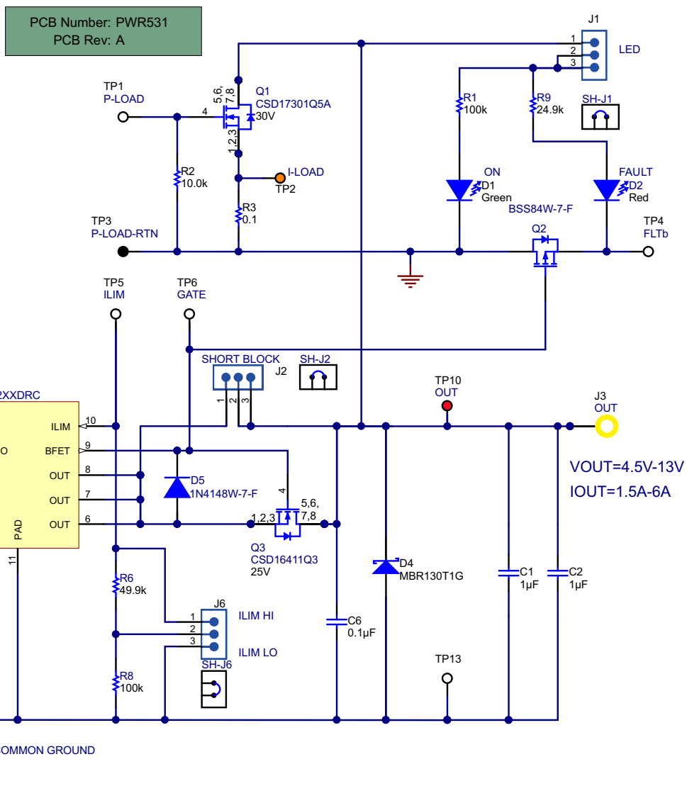
Figure 2-1. TPS2592XXEVM Schematic
