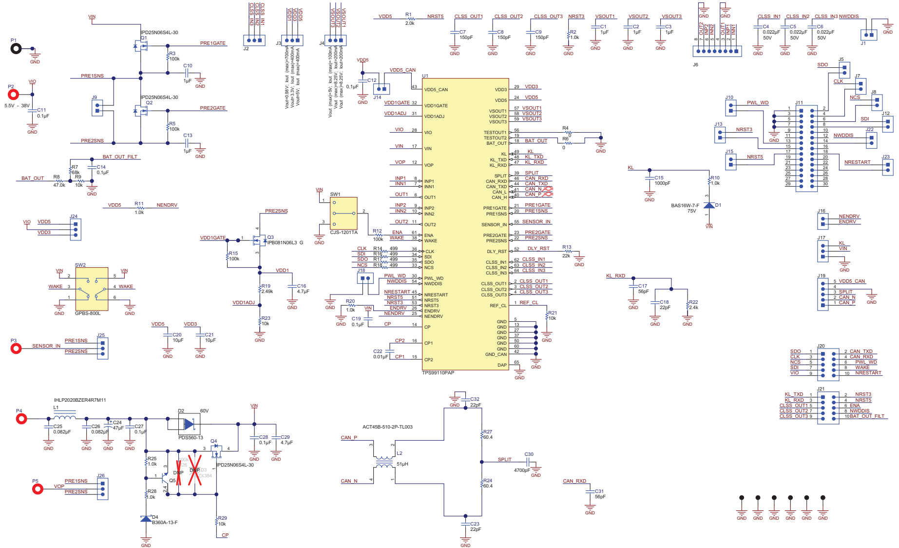
Figure 5. TPS99110EVM Schematic
