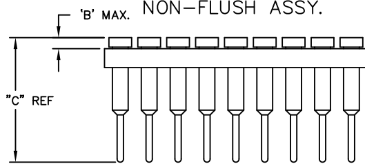
FIGURE 2 NON-FLUSH ASSY.
