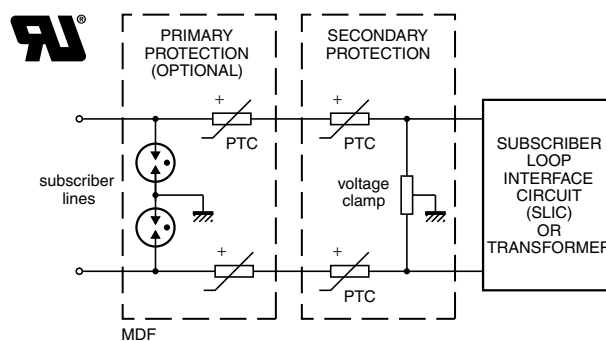
Fig. 1 - Typical telephone line showing where PTC thermistors can be used for overcurrent protection.
