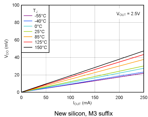
Figure 5-6. Dropout Voltage vs Output Current New silicon, M3 suffix
