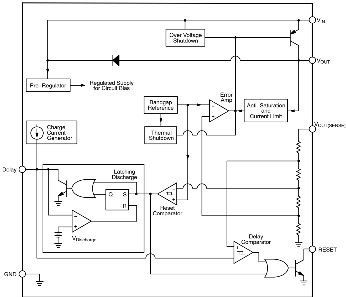
Figure 1. Block Diagram
